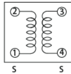
Schematics
